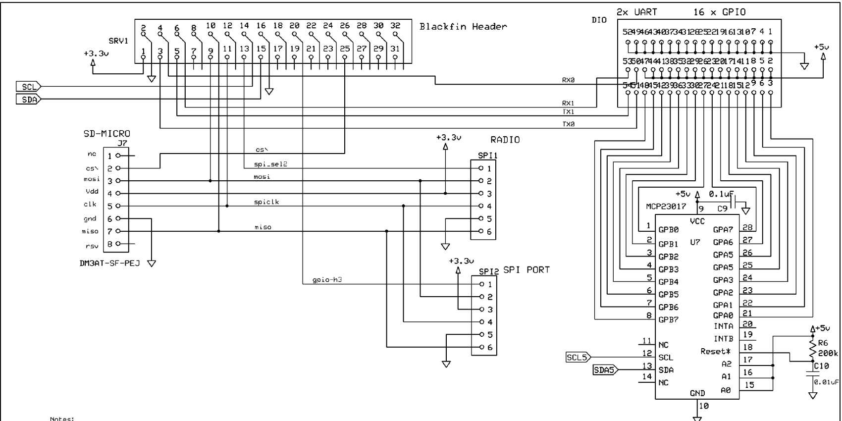
SRV-1- RCM Robot Control Module Schematic Page 2 of 3
